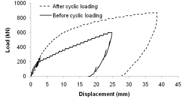
Figure 13. Load vs. displacement before and after cyclic loading for RG-HSP-1.
