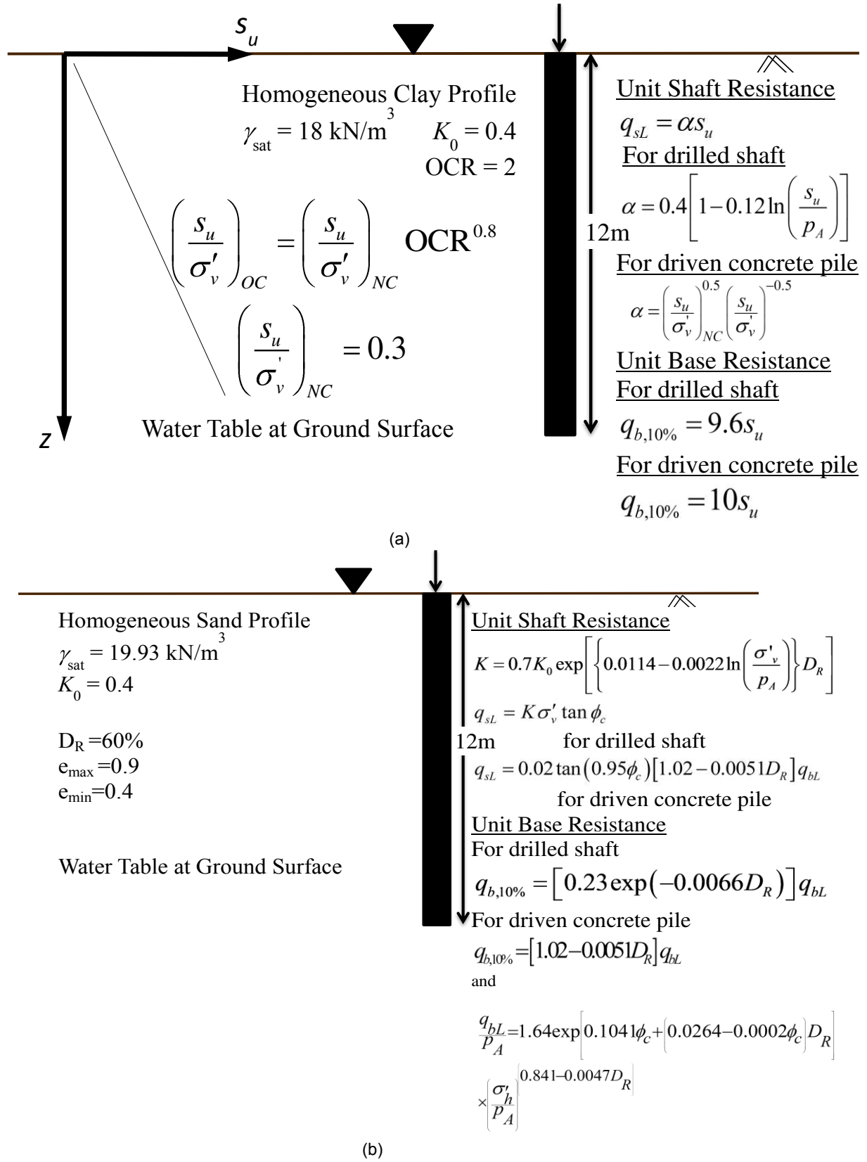
Figure 2. Soil Data and design equations for (a) homogeneous clay and (b) homogeneous sand layers
