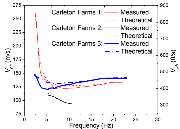
Figure 15. Dispersion curves at Carleton Farms landfill
