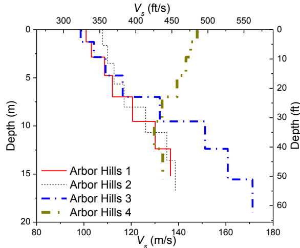
Figure 9. V_s profiles at Arbor Hills landfill
