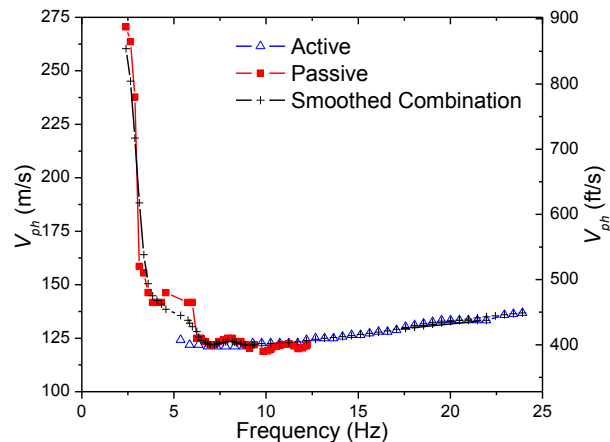
Figure 7. Combination of active and passive dispersion curves (Carleton Farms landfill, location 1)
