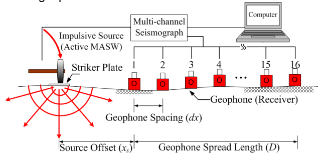
Figure 1. General test setup for MASW
