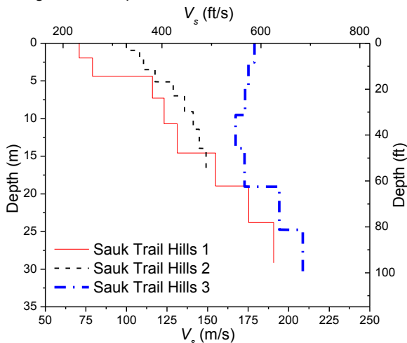
Figure 14. V_s profiles at at Sauk Trail Hills landfill
