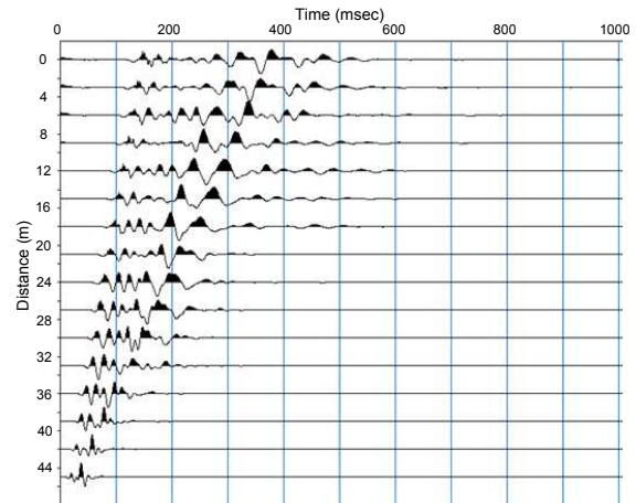
Figure 3. Example of an active record from Carleton Farms landfill location 1.
