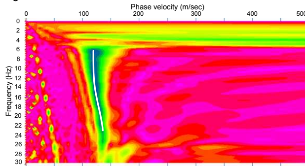
Figure 5. Dispersion curve from MASW data at Carleton Farms landfill location 1
