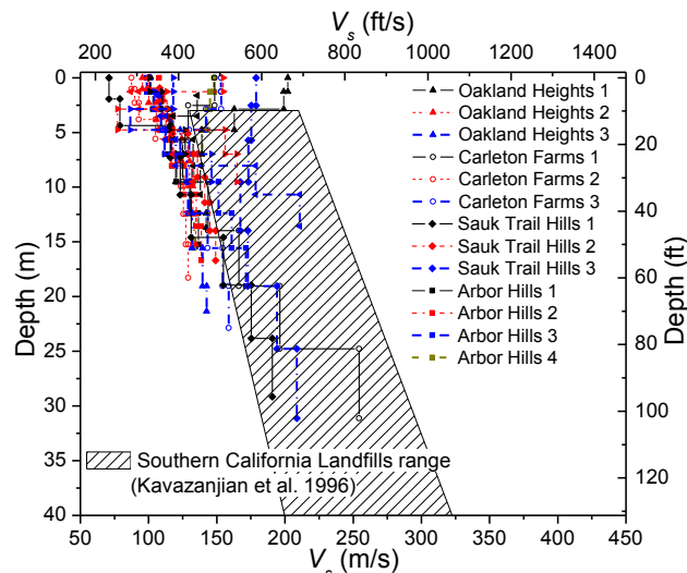
Figure 17. V_s profiles from this study and literature
