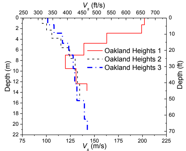
Figure 11. V_s profiles at Oakland Heights landfill
