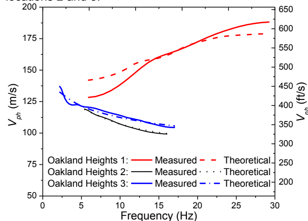
Figure 10. Dispersion curves at Oakland Heights landfill
