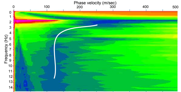
Figure 6. Dispersion curve from MAM data at Carleton Farms landfill location 1
