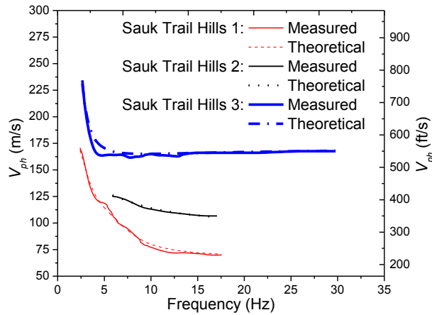
Figure 13. Dispersion curves at Sauk Trail Hills landfill
