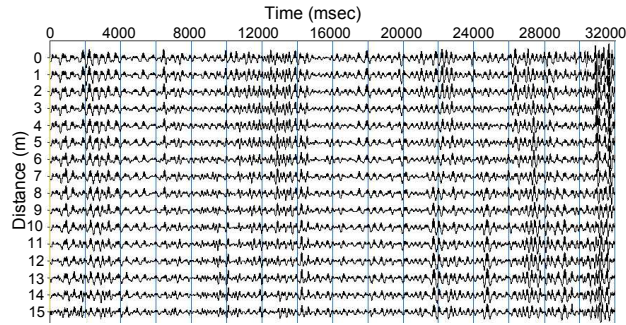
Figure 4. Example of a 32-second passive record at Carleton Farms landfill location 1
