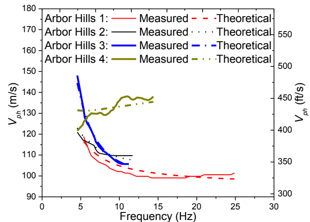
Figure 8. Dispersion curves at Arbor Hills landfill
