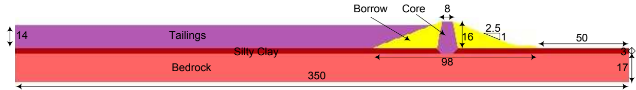
Figure 3: Model geometry (dimensions in meters)
