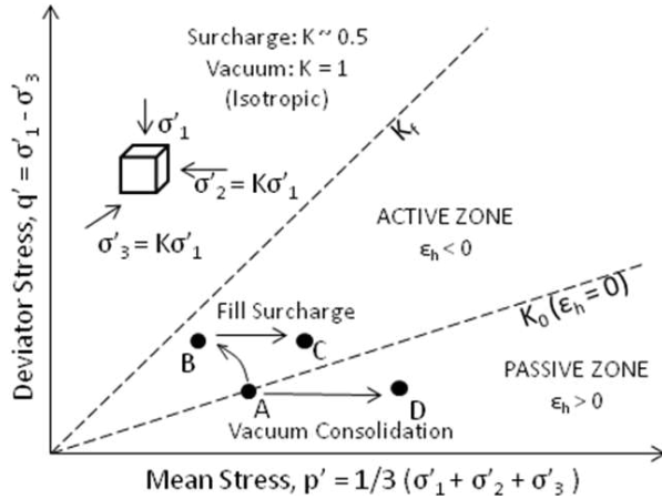
Figure 4. Vacuum on q-p diagram (modified after Spaulding et al. 1993)
