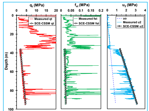
Figure 5. Fitted CPTu profiles at GEB South-II.
