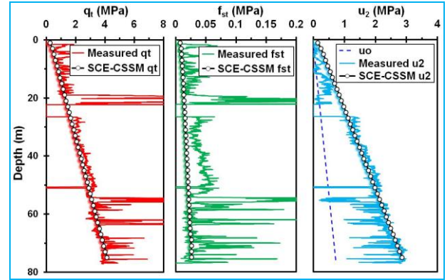
Figure 3. Fitted CPTu profiles at GEB North side.
