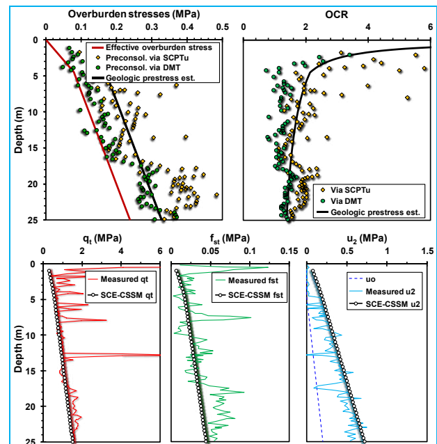
Figure 7. Fitted OCR and CPTu profiles at High Prairie.
