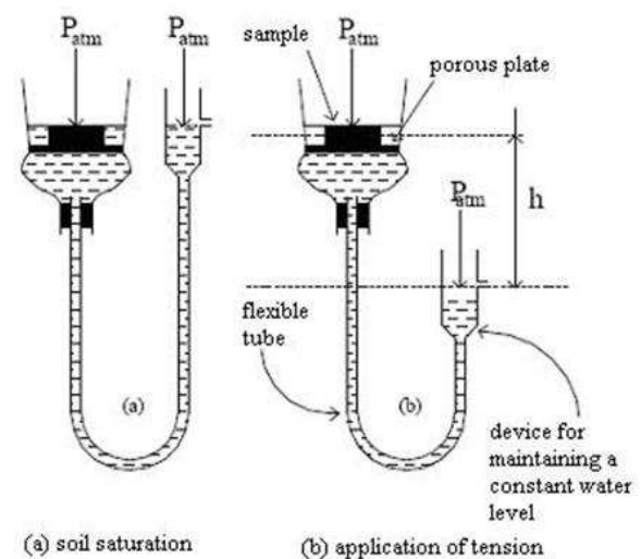
Figure 3. Illustration of Haines funnels equipment.
