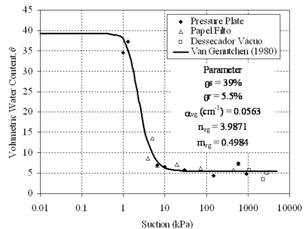
Figure 6. Soil-water characteristic curve adjusted by Van Genuchten (1980) – Barreiras Formation Coutinho et al. (2006).
