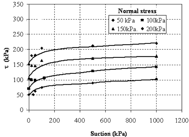
Figure 9. Shear strength envelopes in the space ( s , \tau ) adjusted according to the hyperbolic function used by Gens (1993) –residual soil of granite – research area 2.
