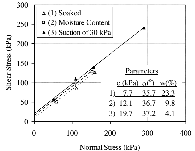
Figura 10. Shear strength envelopes – direct shear test, Barreiras Formation – Coutinho et al. (2006)
