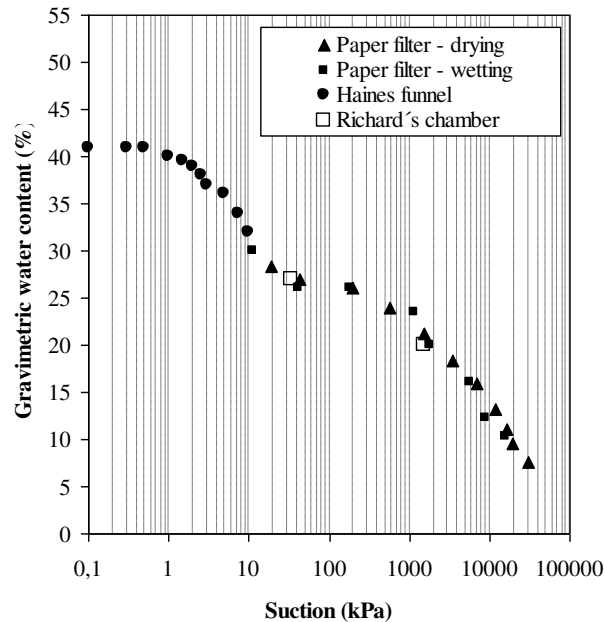
Figure 4. Soil-water characteristic curve research area 1 - Silva & Coutinho (2007).
