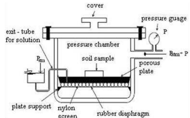
Figure 2. Richard's Pressure Chamber.
