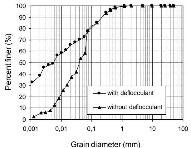
Figure 1. Granulometric test results – area 1.
