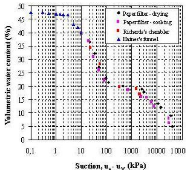
Figure 5. Soil water characteristic curve – area 2, Lafayette (2006).
