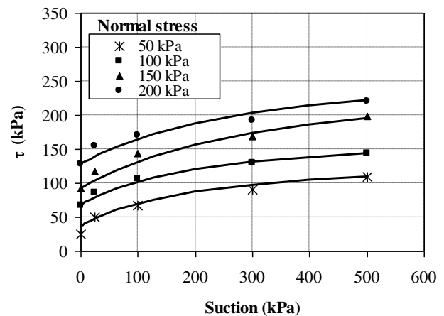
Figure 8. Shear strength envelopes in the space ( s , \tau ) adjusted according to the hyperbolic function used by Gens (1993) – residual soil area 1.
