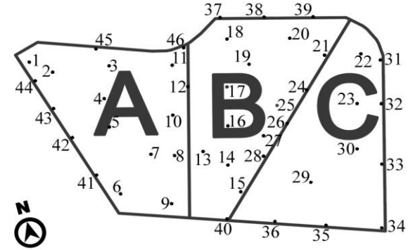
Figure 10. Survey points.
