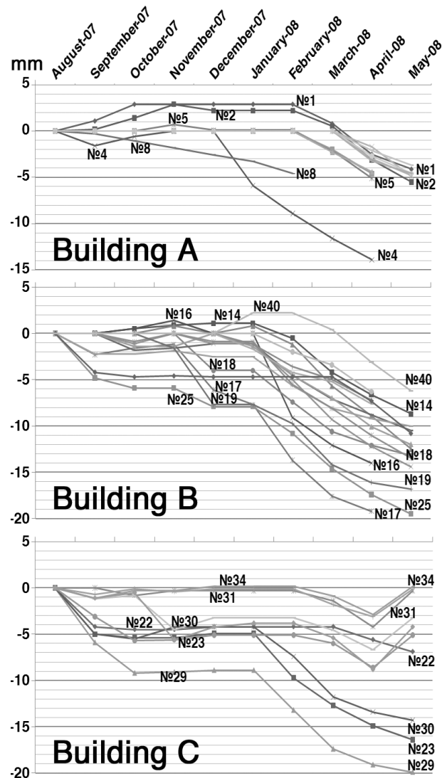
Figure 11. Settlement survey of buildings.
