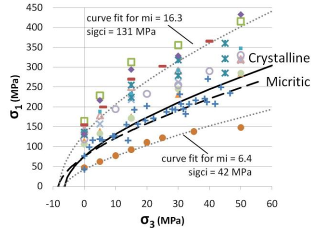
Figure 5: Triaxial carbonate data (courtesy of Dr. Evert Hoek) with curves used in the numerical modeling
