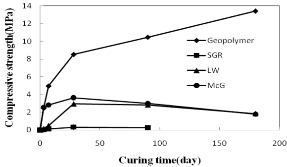
(a) Long geltime specimens (gel time 60~120sec)
