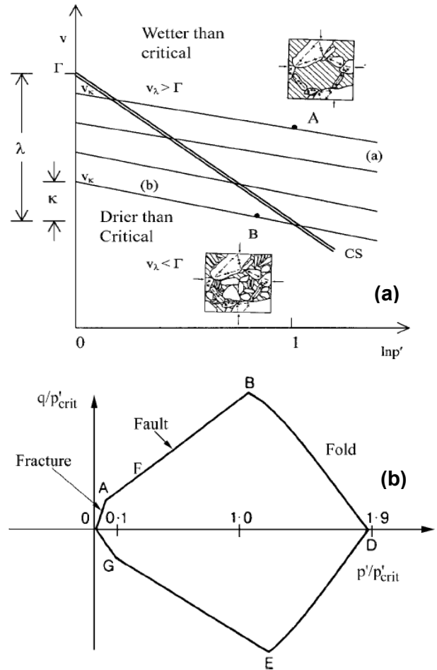
Figure 2. Concepts of CSSM used to differentiate soil states (a) Compression and swelling of soils. (b) Limits of stable states of yielding in the modified stress space (Muhunthan and Schofield, 2000)
