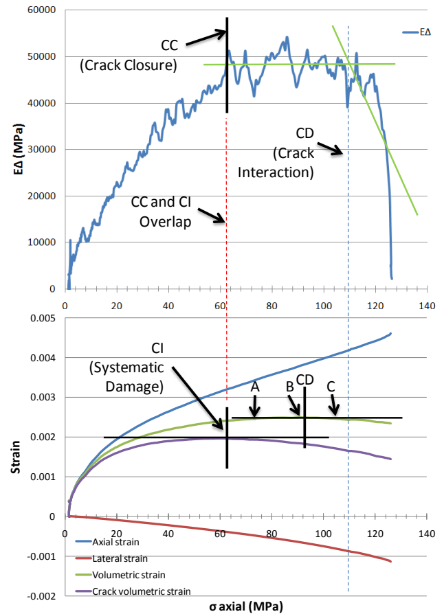
Figure 15. Detection of CI and CD for the Stanstead granite sample using tangent modulus (EΔ), volumetric strain and crack volume strain methods.
