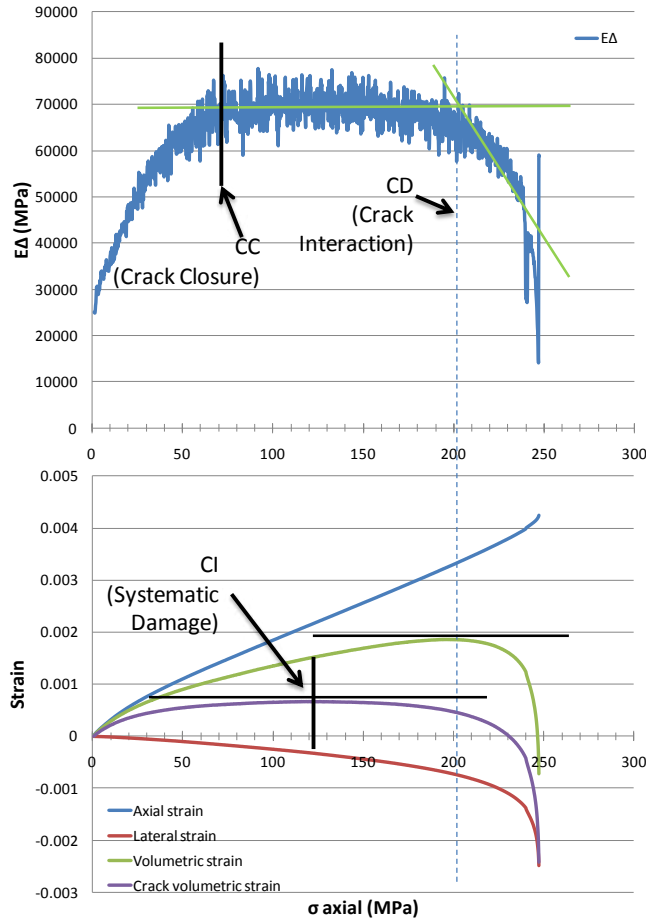
Figure 13. Detection of CI and CD for the Smaland granite sample using tangent modulus (EΔ), volumetric strain and crack volume strain methods.
