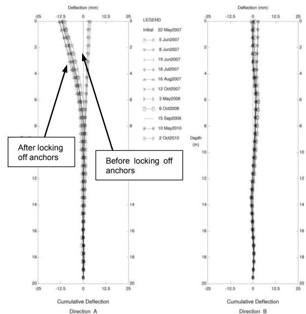
Figure 5. Incremental and cumulative deflection versus depth plots for the Lindbergh Hill wall
