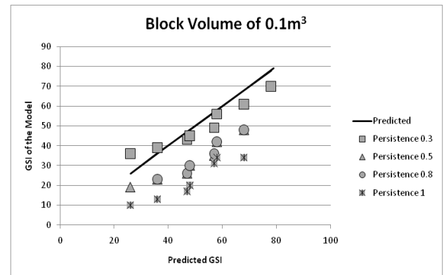
Figure 8. 45cm block size with correction of block volume according to Cai et al 2004.
