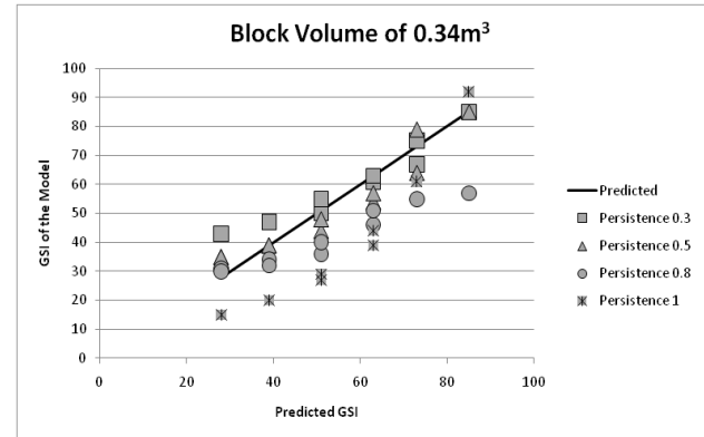
Figure 7. 70cm block size with correction of block volume according to Cai et al 2004.
