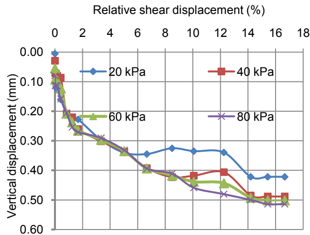
Figure 6: Vertical displacement vs relative shear displacement for water content of 59%
