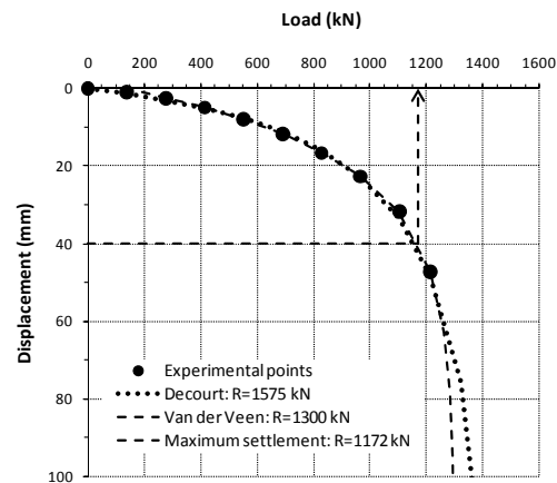
Figure 9 Extrapolating curves for the groups of two piles
