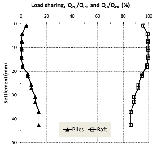
Figure 7 Measurement of load sharing between piles and raft
