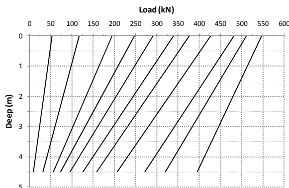
Figure 8 Load transfer to soil by skin friction and the pile tip
