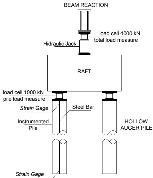
Figure 4. Instrumentation scheme
