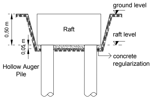
b) Piled Raft
