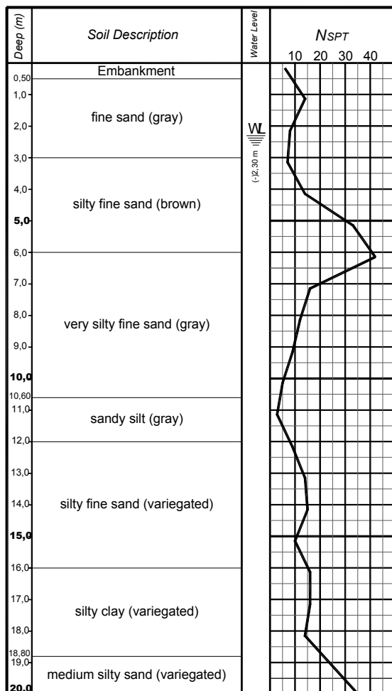
Figure 1 Standard Penetration Test
