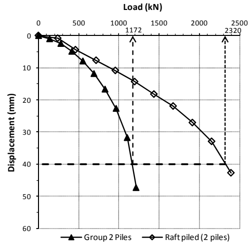
Figure 11 bearing capacity of foundations
