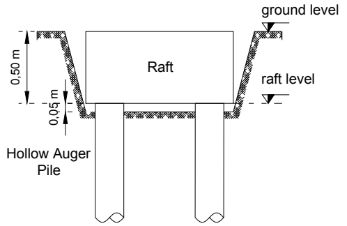
a) Pile Group
