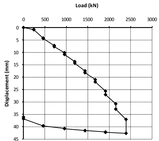
Figure 6 Load x settlement curve for piled raft with two piles
