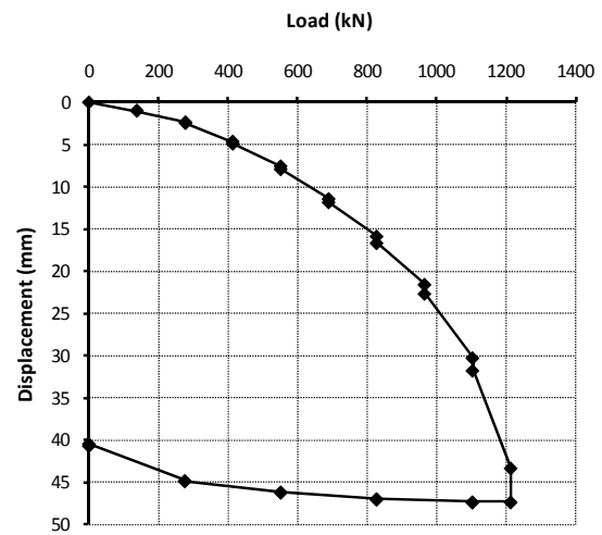
Figure 5 Load x settlement curve for two piles groups
