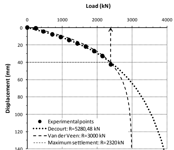
Figure 10 Extrapolating curves for 2-piled raft
