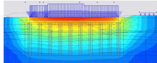
Equivalent soil block approach
