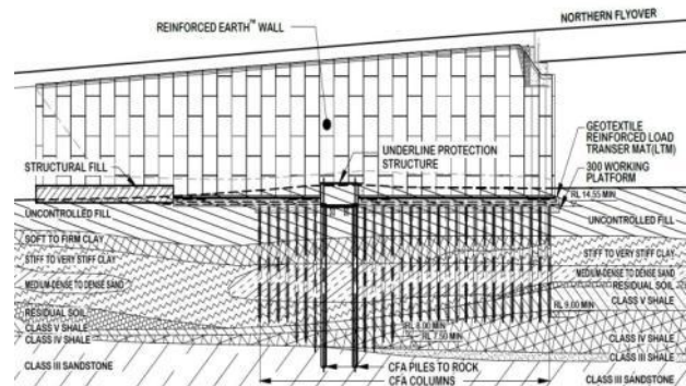
Figure 2. Surface profile and ground improvement
