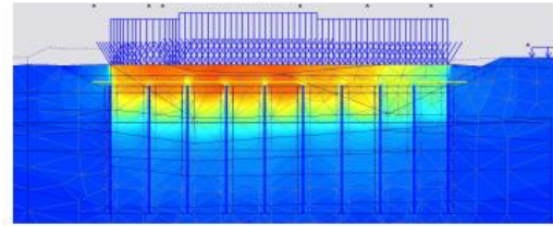
Plate element approach
