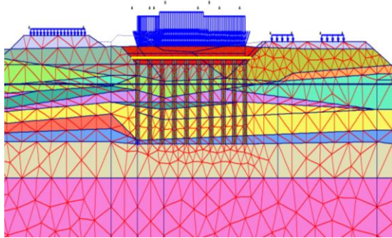
Figure 8. PLAXIS Model: Transverse Direction (Concrete Column as Soil Elements)
