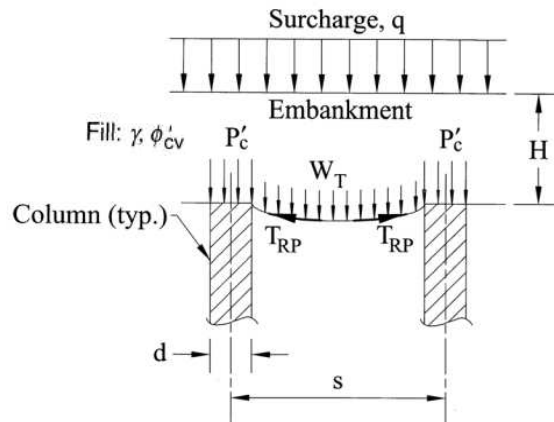
Figure 5. Variables as defined by BS 8006
