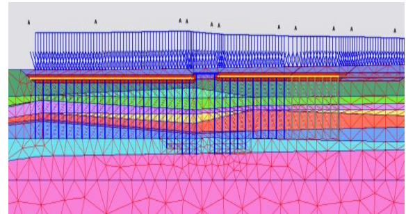
Figure 7. PLAXIS Model: Longitudinal Direction (Plate Elements)
