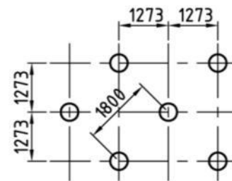
Figure 4. CFA grid pattern and spacing.
