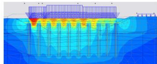
Soil element approach
