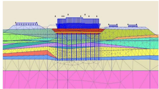
Figure 6. PLAXIS Model: Transverse Direction (Plate Elements)
