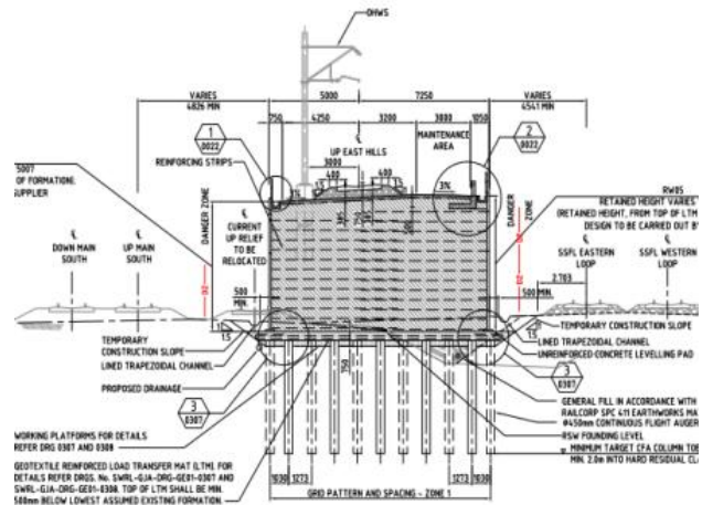
Figure 3. CFA Column Supported Embankment
