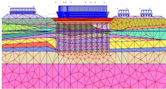
Figure 9. PLAXIS Model: Transverse Direction (Equivalent Soil Block)
