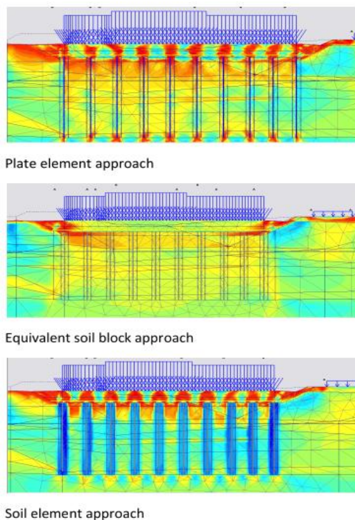
Figure 12. Relative shear stress plots
