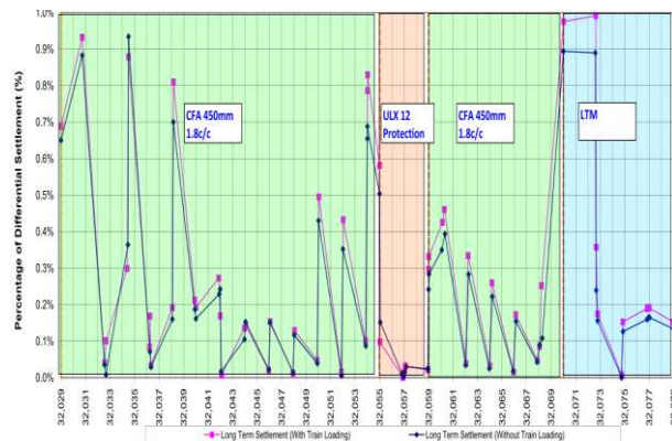
Figure 11. Differential Settlement within ground treatment zone by CFA
