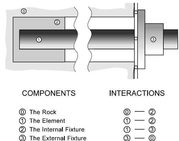
Figure 1. Generic reinforcement system.
