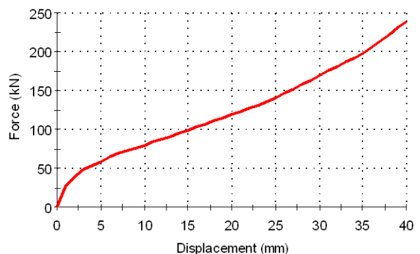
Figure 22. Total shear force-displacement response.
