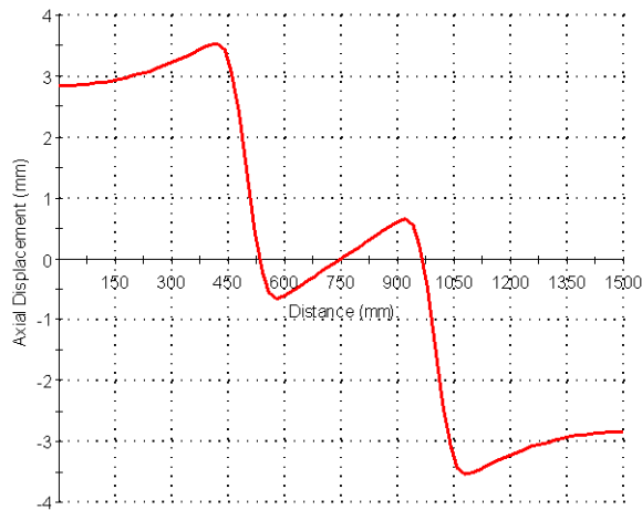
Figure 18. Distribution of axial displacement relative to the borehole.
