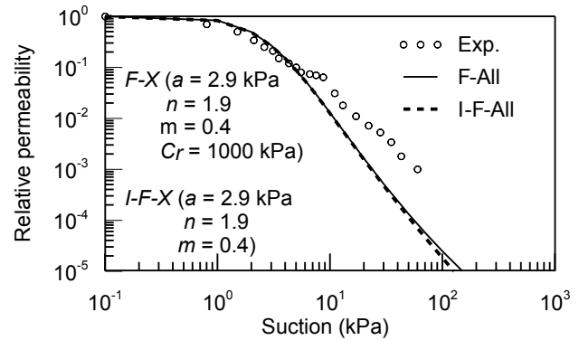
Figure 16. F-All and I-F-All models for Yolo light clay
