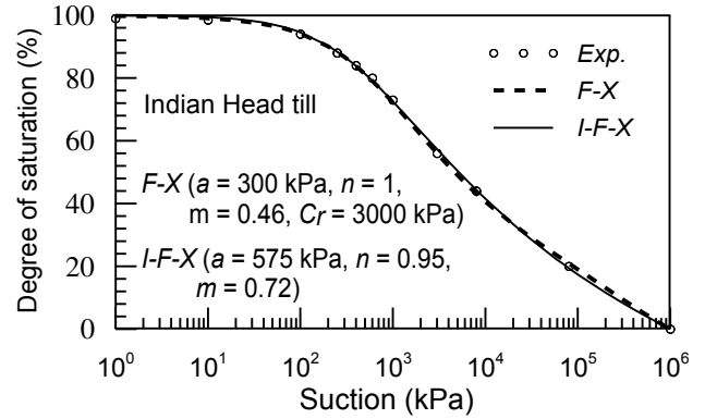
Figure 12. F-X and I-F-X SWCCs for Indian head till
