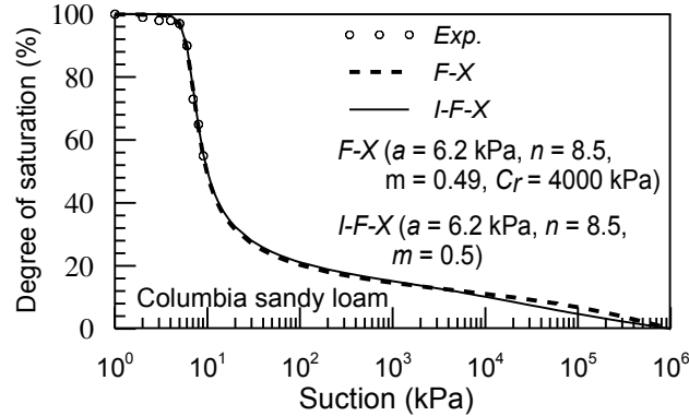
Figure 9. F-X and I-F-X SWCCs for Columbia sandy loam
