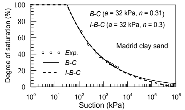
Figure 2. B-C and I-B-C SWCCs for Madrid clay sand
