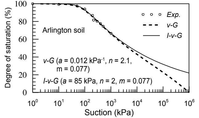
Figure 7. v-G and I-v-G SWCCs for Arlington soil
