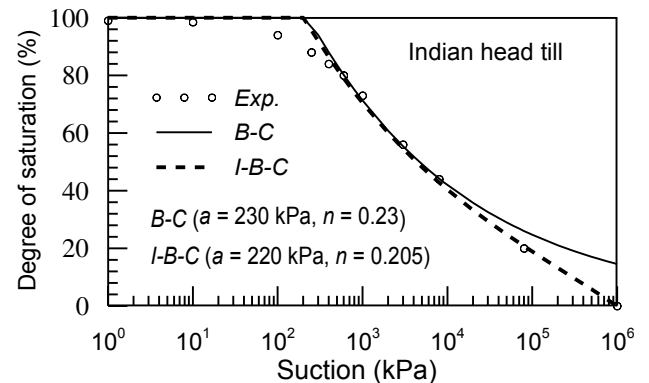
Figure 4. B-C and I-B-C SWCCs for Indian head till
