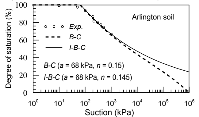
Figure 3. B-C and I-B-C SWCCs for Arlington soil
