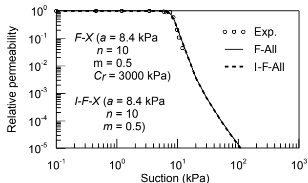
Figure 15. F-All and I-F-All models for Touchet silt loam
