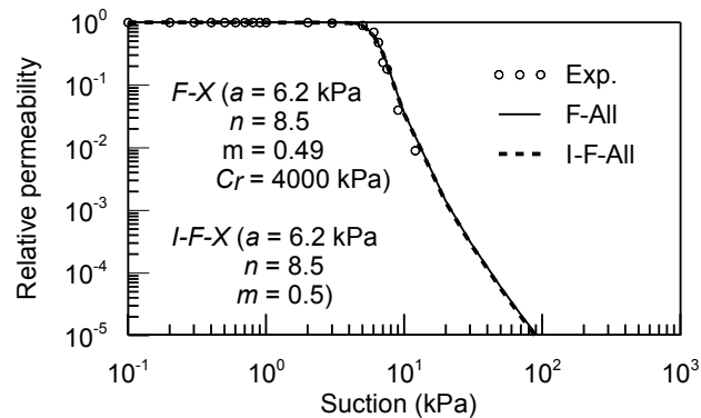
Figure 14. F-All and I-F-All models for Columbia sandy loam
