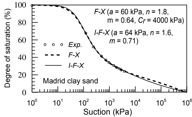
Figure 10. F-X and I-F-X SWCCs for Madrid clay sand
