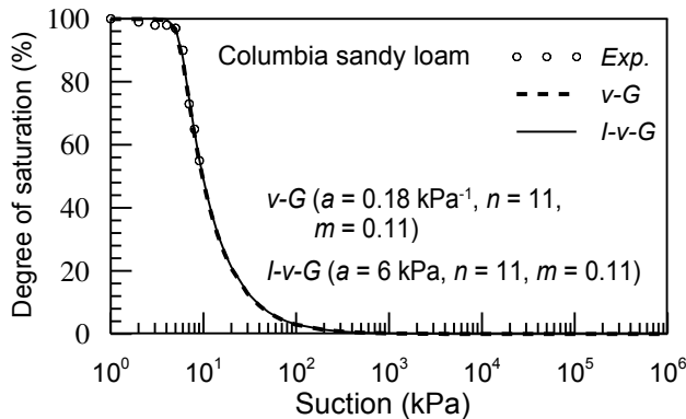
Figure 5. v-G and I-v-G SWCCs for Columbia sandy loam
