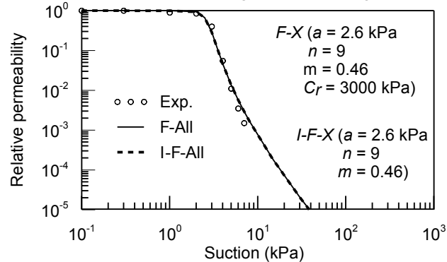
Figure 13. F-All and I-F-All models for Superstition sand
