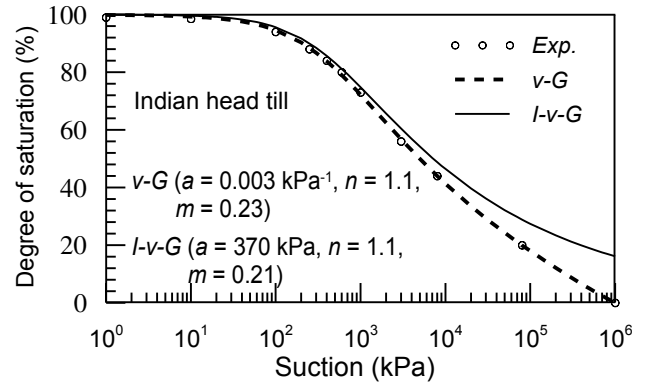
Figure 8. v-G and I-v-G SWCCs for Indian head till
