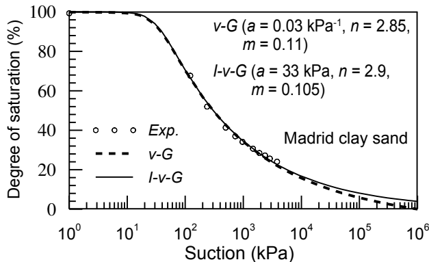
Figure 6. v-G and I-v-G SWCCs for Madrid clay sand
