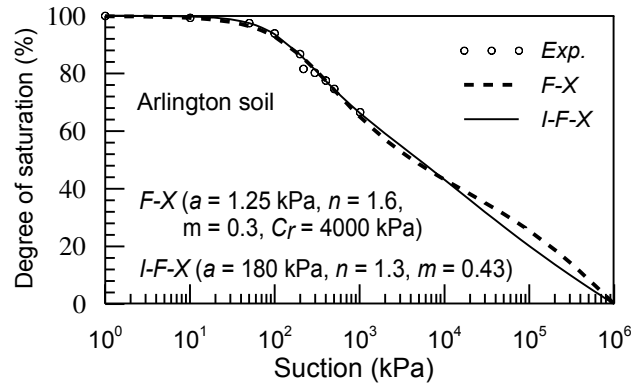
Figure 11. F-X and I-F-X SWCCs for Arlington soil
