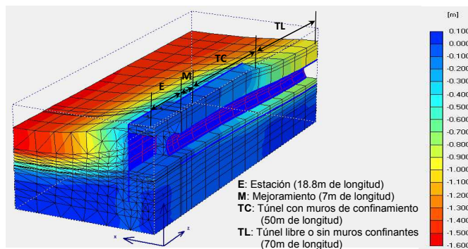
Figure 6. Deformed 3D finite elements mesh for the study of the definition of the confining wall length.
