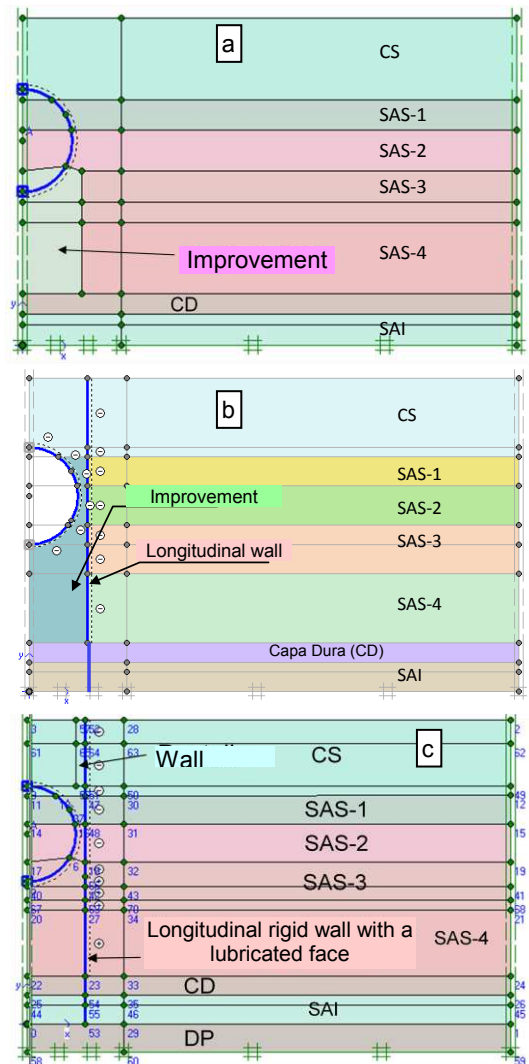
Figure 3. Conceptual models with 2D FEM, to study solution with bottom improvement (a), longitudinal walls and improvement (b), and longitudinal walls and superficial screen (c).
