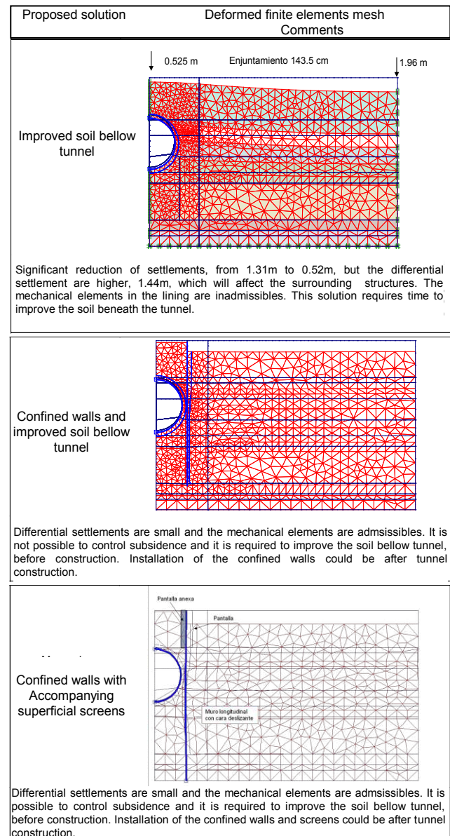
Figure 5. Deformed finite elements mesh for the various proposed solutions, and their respective comments.
