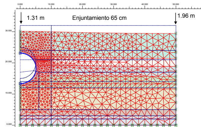
a) Deformed mesh
