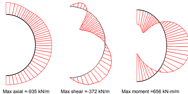
b) Mechanical elements on lining
