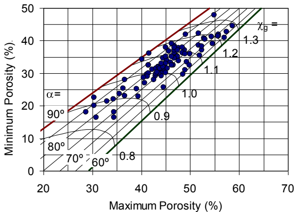
Figure 5. Maximum porosity versus minimum porosity diagram. The experimental data were reported by several authors. The lower straight line stands for the tetrahedral packing, and the higher, for the octahedral one.
