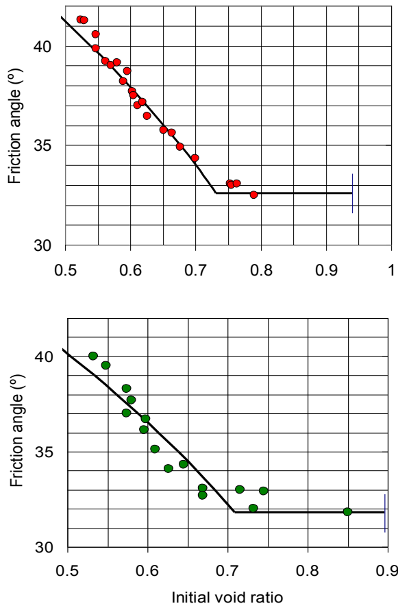
Figure 10. Relationship between the initial void ratio and the friction angle. a) for Brasted sand, x_g=1.016 , (Cornforth, 1973) , b). for medium fine sand, x_g= 0.993 , (Rowe,1962),
