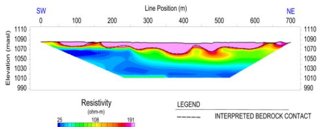
Figure 6 Electrical Tomography results – Line 4
