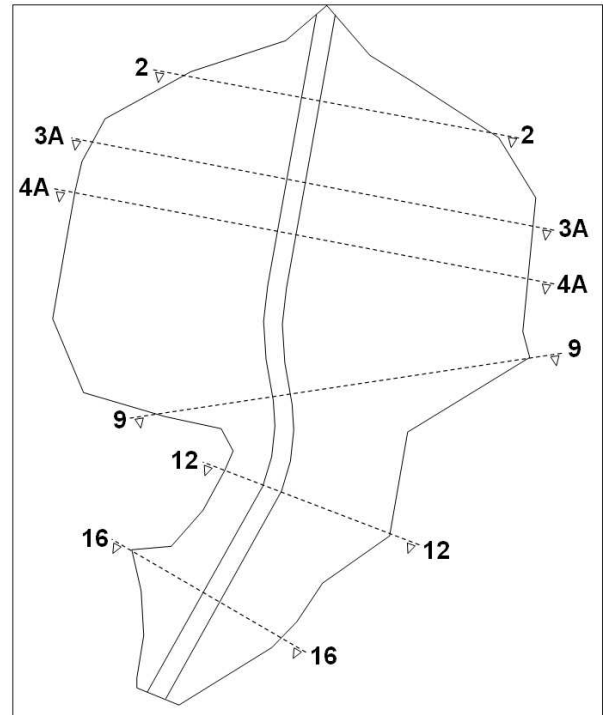
Figure 2. Layout of the Doosti dam and locations of the sections selected
