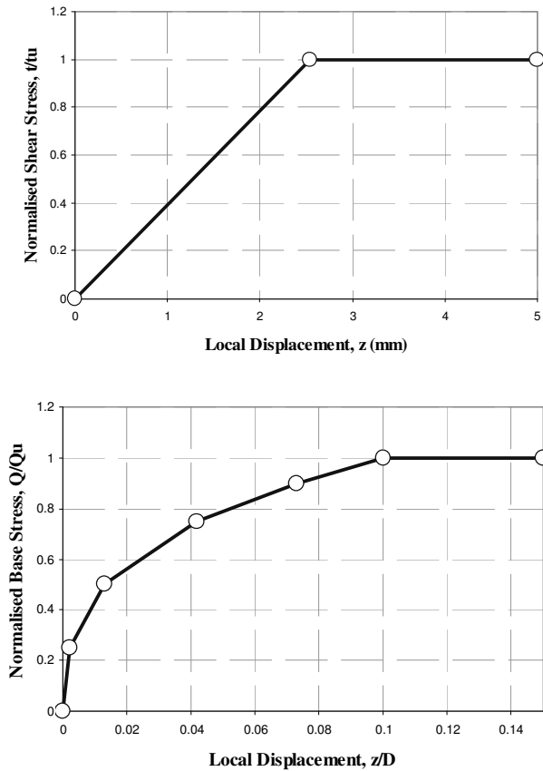
Figure 2a: t-z curves and (b) Q-z curves assumed in the analysis
