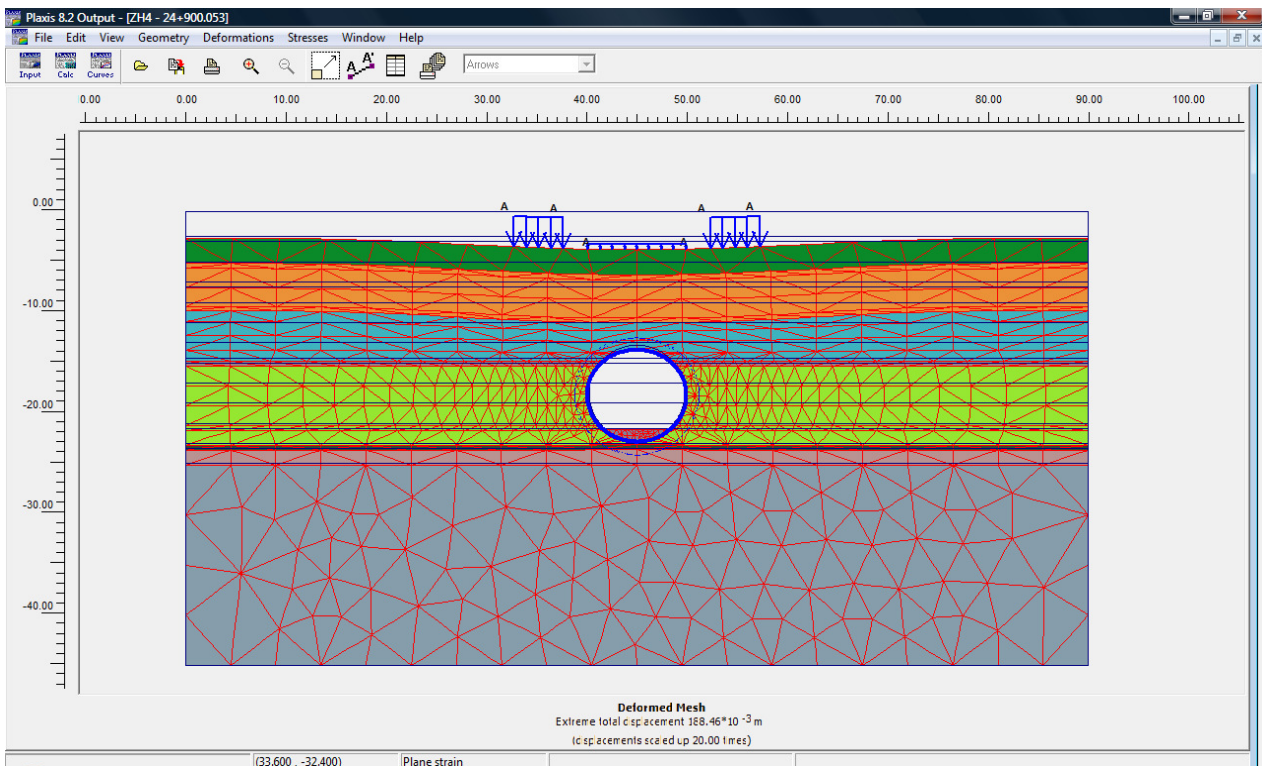
Figure 4. 2D finite element model of tunnel lining
