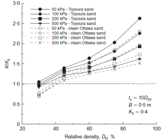
Figure 1. Effect of initial effective vertical stress and relative density on K/K_0 (Loukidis and Salgado 2008)
