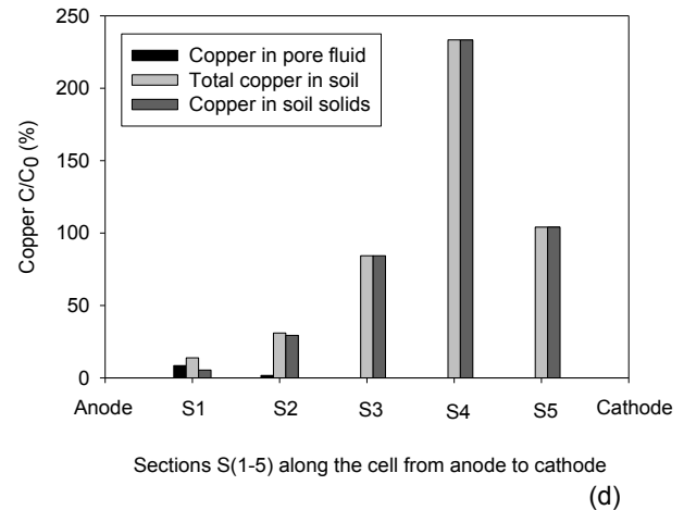
Figure 8. Copper concentration after the tests in sections S1 to S5 for (a) clay-sand mixture (b) clay with sand buckets, (c) clay-sand layers, and (d) homogenous clay.
