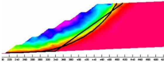
Figure 9 – Displacement field and two potential rupture surfaces from finite element analysis ( FS_{static} = 1.60 ).
