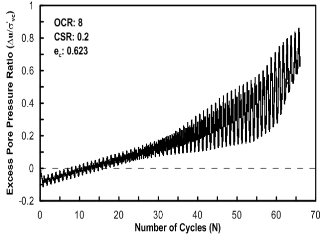
Figure 8. The Excess pore pressure generation for OCR_M = 8
