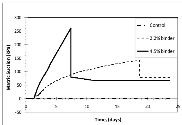
Figure 5 Self-desiccation tests for Kidd tailings
