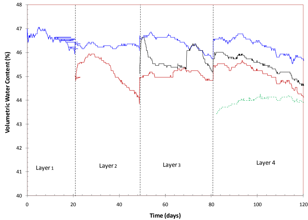
Figure 8 Volumetric water contents measured in column test
