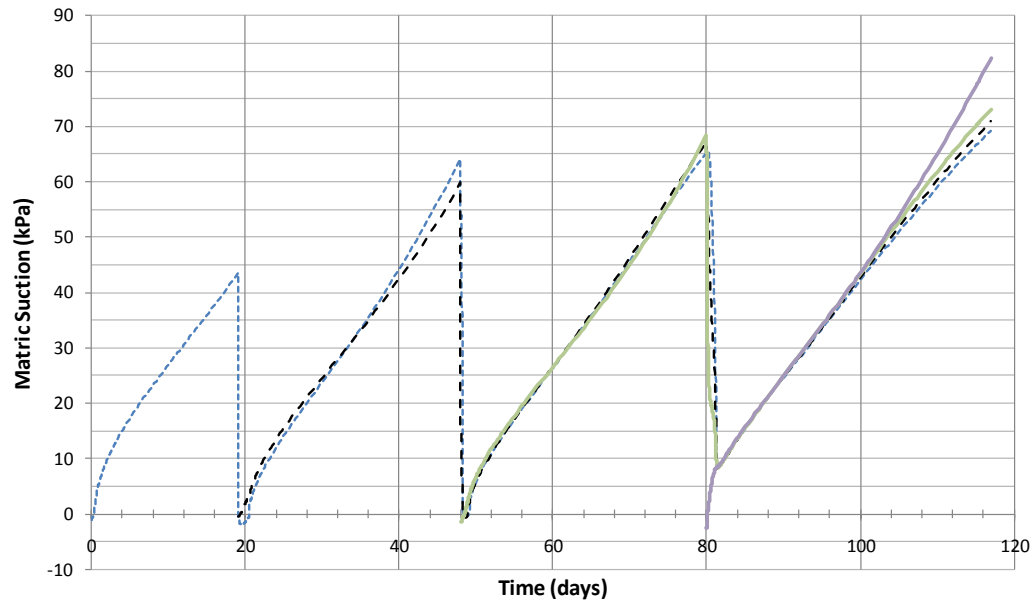
Figure 9 Simulated matrix suction values in column test, each line corresponds to a mid-layer prediction (4 layers)
