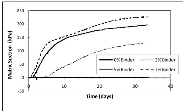
Figure 4 Self-desiccation tests for Williams tailings
