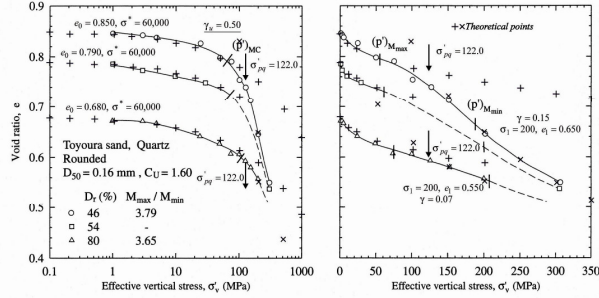
Figure 17. Type A compression behavior of Toyura sand in isotropic compression (data from Kwag et al. 1999). (p')MC, equal all-around pressure at yield point defined at the point of maximum curvature of e versus \log p' ; (p')M max , equal all-around pressure at yield point defined at first inflection point of maximum curvature of e versus \log p' ; (p')M min , equal all-around pressure at the second inflection point of e versus p' defining end of the second stage of compression
