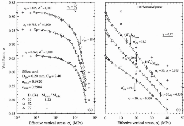
Figure 18. Compression behavior of Silica sand used to study secondary compression (data from Yet. 1998)
