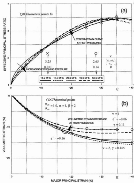
Figure 12. Compression Tests between 15.0 and 52.0 Mpa Confining pressures for Dense Cambria Sand: (a) Effective Principal Stress Ratio; and (b) Volumetric Strain Relations (from Yamamuro and Lade. 1996)
