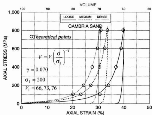
Figure 3. Axial Stress Related to Axial Strain for One-Dimensional Compression Tests on Cambria Sand (from Yamamuro et al. 1996)
