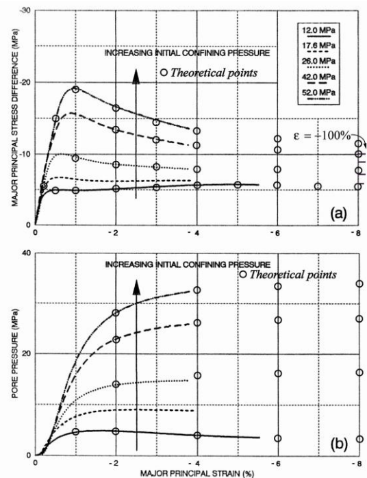
Figure 9. Undrained Extension Tests Between 12.0 and 52.0 MPa Initial Confining Pressures on Dense Cambria Sand: (a) Principal Stress Difference; and (b) Pore Pressure Relations (from Lade and Yamamuro, 1996)
