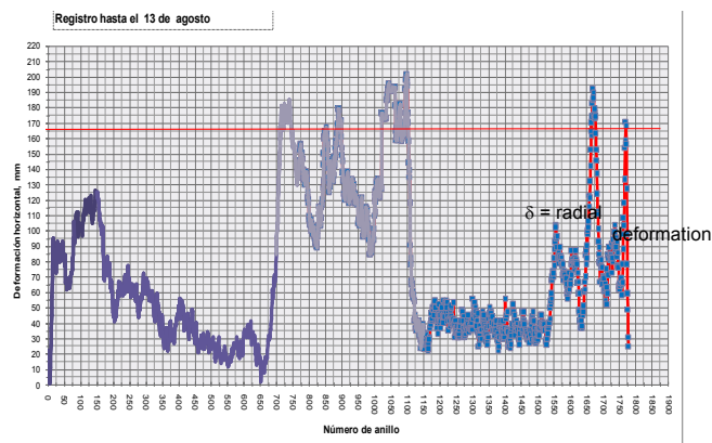
Figure 3. Horizontal deformation measurements in dowel rings (Meza and Auvinet, 2010).
