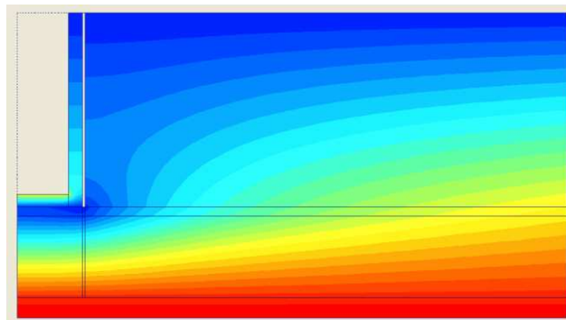
Figure 11. Modeling of pumping in the permeable layer to control uplift pressure.
