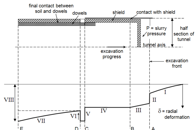
Figure 1. Double ring model (Maidl and Comulada, 2010).
