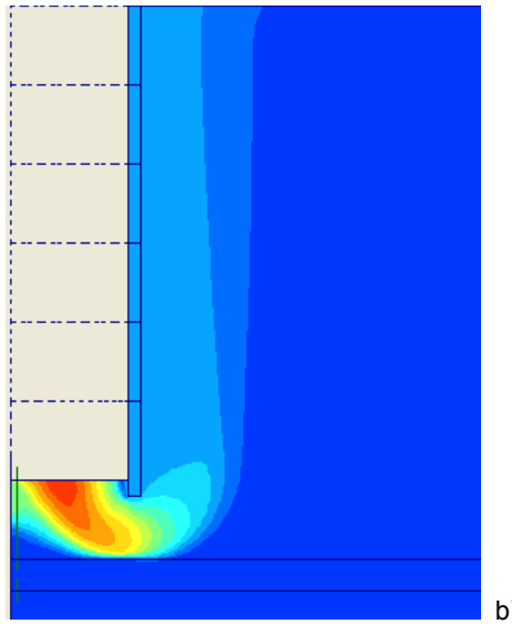
Figure 7. Potential shear failure mechanisms a) without perimetral mortar wall b) with mortar wall
