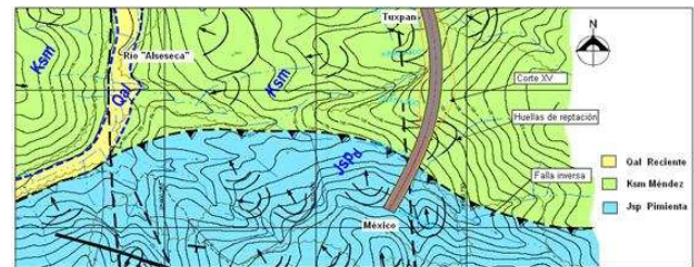
Figure 1. Topographic location of Cut XV
