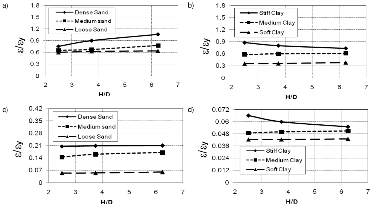
Figure 5. Effect of embedment ratio on maximum axial strain at elbow of buried pipe in different soil ( D=0.4\text{m} , t=0.0095\text{m} ); a) sand, Chichi earthquake, b) clay, Chichi earthquake, c) sand, Northridge earthquake, d) clay, Northridge earthquake.
