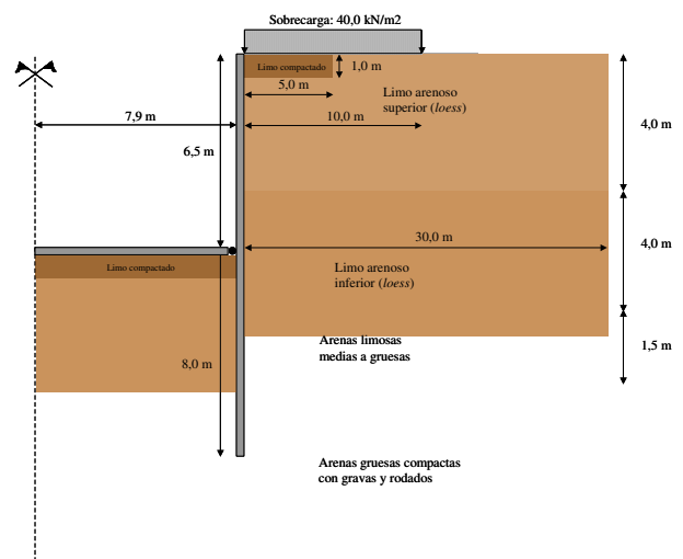
Figure 7. Structure profile
