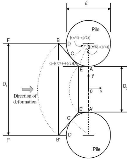
Figure 1. Elastoplastic model from Ito and Matsui.
