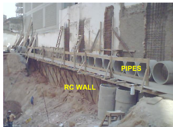
Picture 1. Reinforced Concrete wall and pipes employed to excavate the piles.
