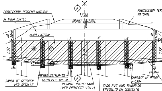
Figure 6. Contiguous pile wall scheme
