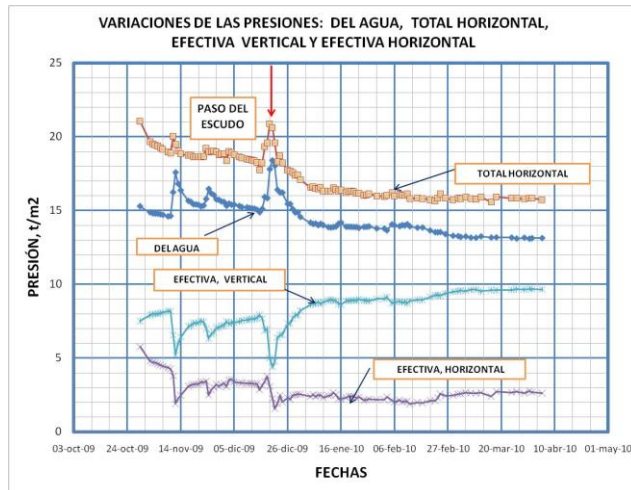
Figure 6. Variations with time of water, total horizontal, effective horizontal and effective vertical pressures
