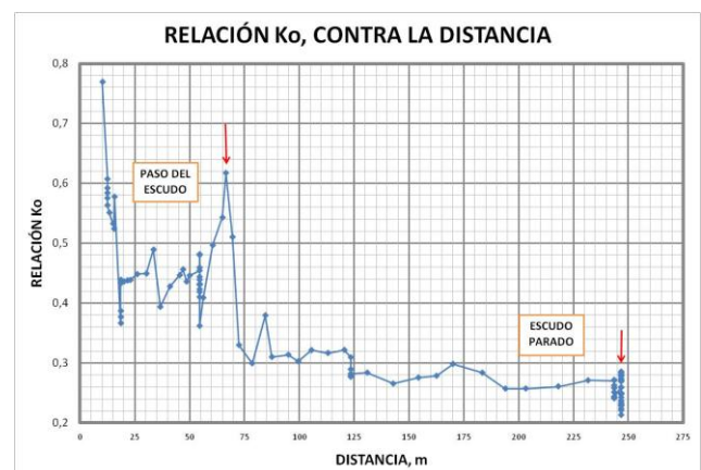
Figure 9. Variation of the k_0 ratio in terms of distance
