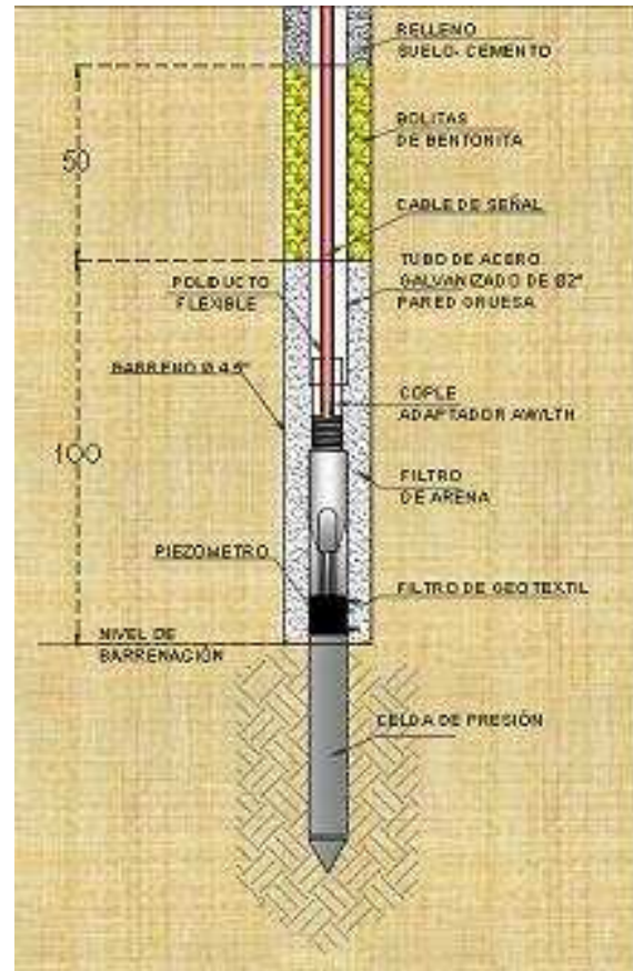
Figure 4. Piezo-cell installed
