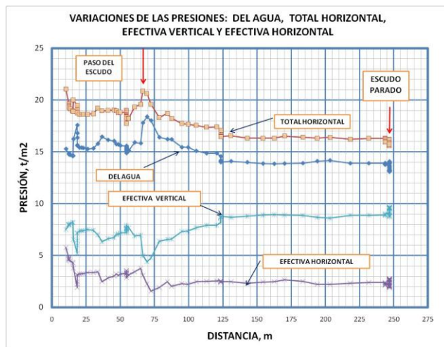
Figure 7. Variations in terms of distance of water, total horizontal, effective horizontal and effective vertical pressures
