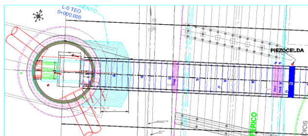
Figure 5. Location in plan of the piezo-cell installed
