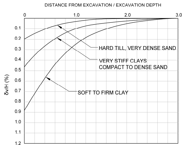
Figure 7. Empirical relationship between ground type and anticipated displacement due to deep excavations (from Boone and Westland 2004)
