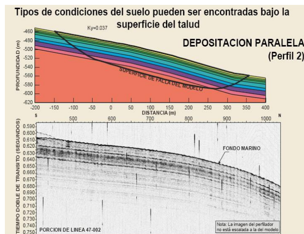
Figure 8. Review stability seabed evaluation process (courtesy Fugro, 2009).
