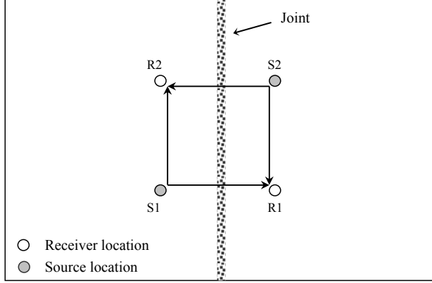
Figure 2. Testing geometry for equal-spacing transmission coefficient method (Jiang 2007).
