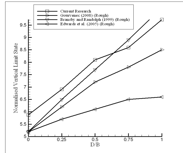
Figure 12. Ultimate vertical bearing capacity as a function of embedment ratio for Yoldia clay
