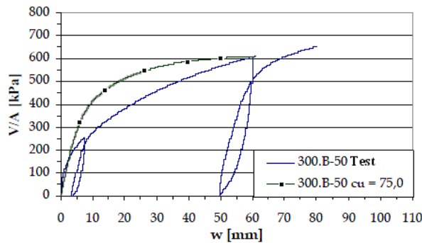
Figure 11. Load-displacement curves for bucket foundation with 30 cm diameter ( E_{25} = 9411 \text{ kPa} )
