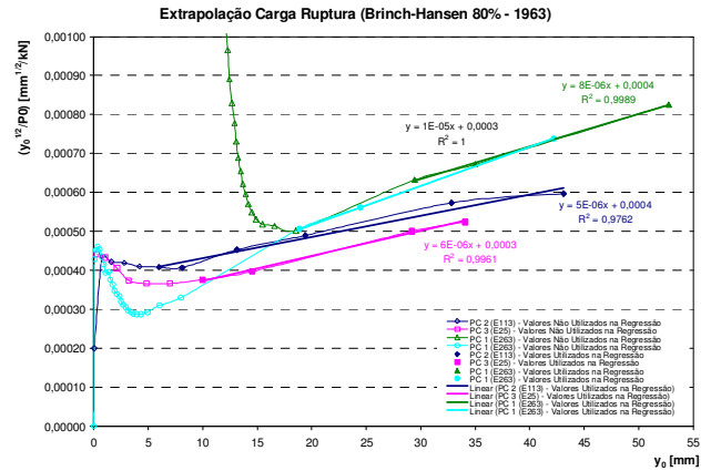
Figure 8. Brinch-Hansen 80% Method.
