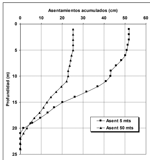
Figure 7. Total settlement estimated at final stage.
