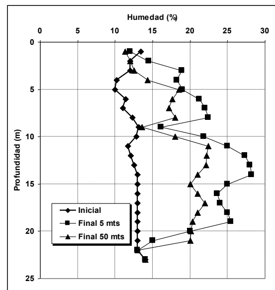
Figure 6. Moisture content profile at initial and final stages
