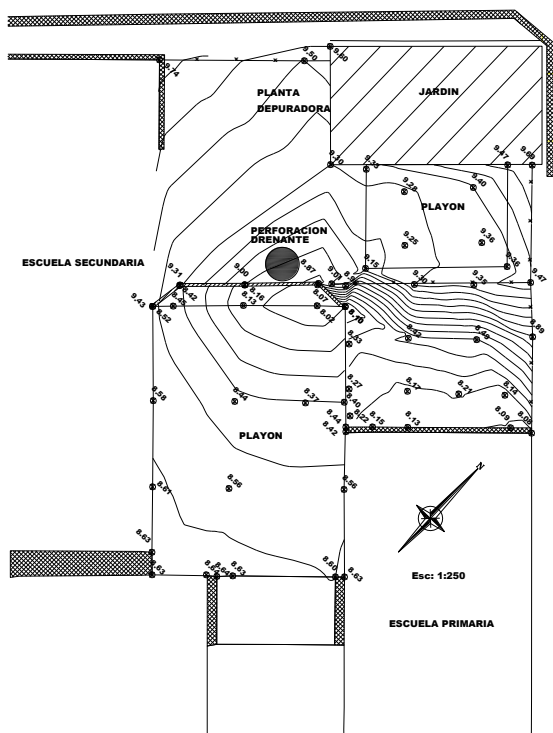
Figure 4. Land survey after subsidence. Souce: Terzariol, 2009.
