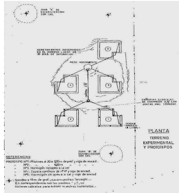
Figure 2. Plan of Prototypes and crater contour. Source: Moll, 1972.
