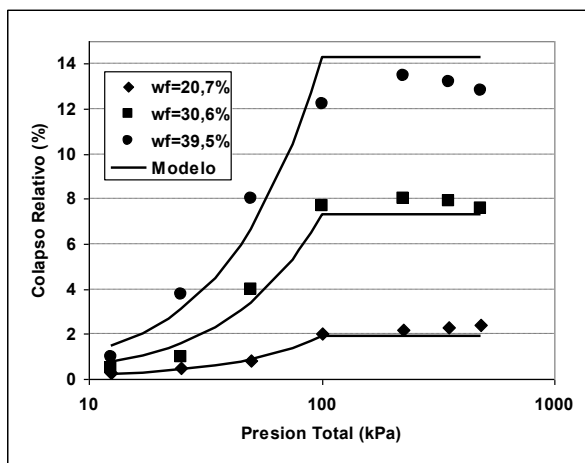
Figure 5. Experimental results of studies on collapse and relative collapse model. Source: Aiassa, 2008
