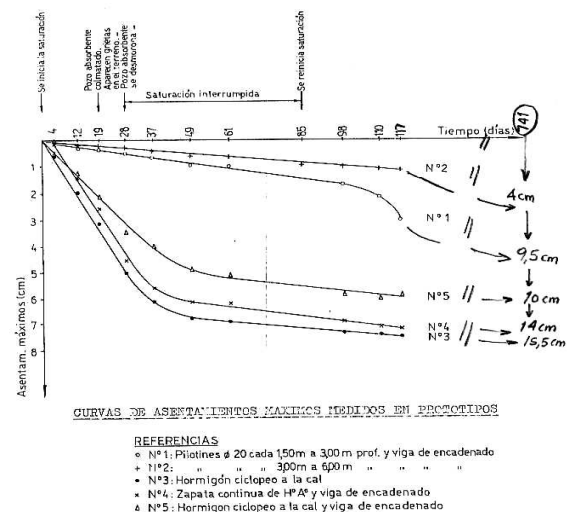
Figure 3. Settlement against time. Source: Moll, 1972.
