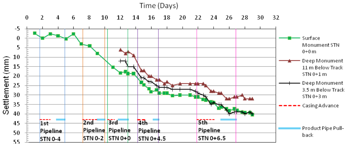
Figure 11: Ground settlement versus time for survey monuments at depth in embankment
