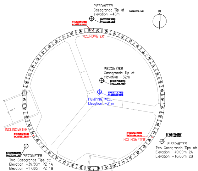
Figure 14. Monitoring system at Access Shaft N° 1
