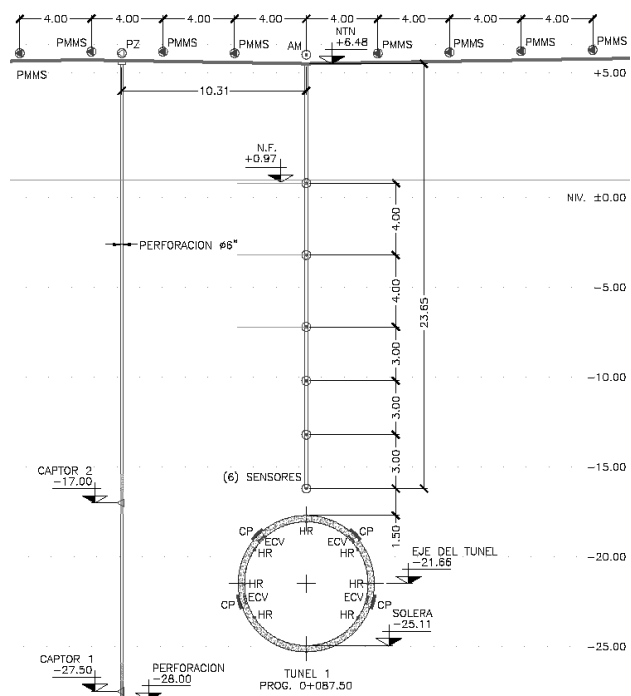
Figure 13. Typical monitoring section
