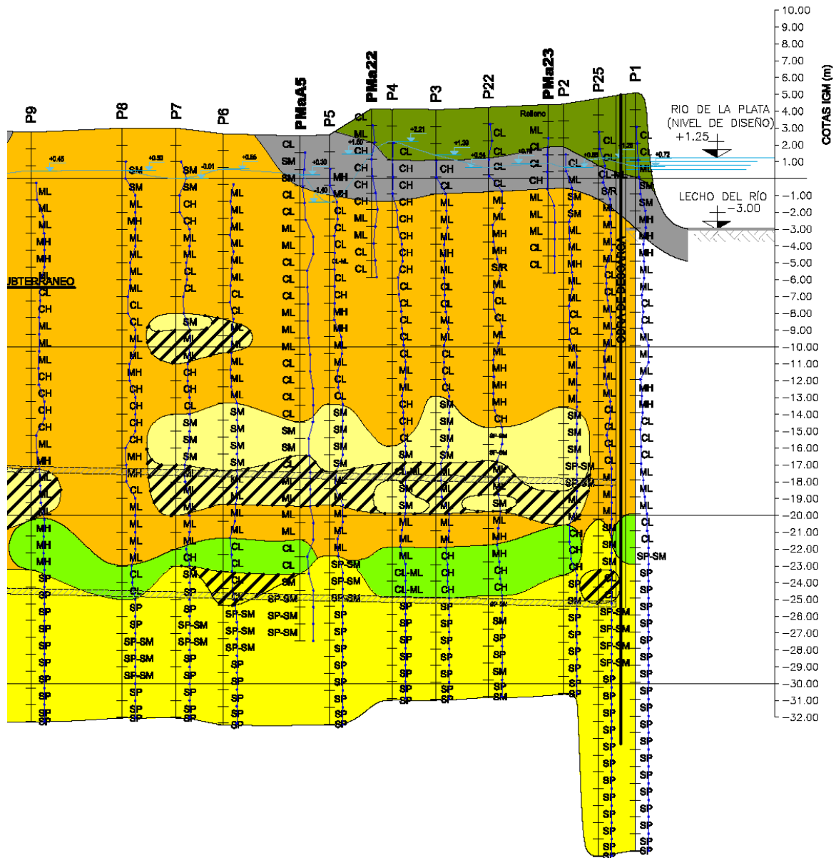
Figure 3. Longitudinal geotechnical profile – Tunnel N° 1 (Short Tunnel), near Access Shaft N° 1
