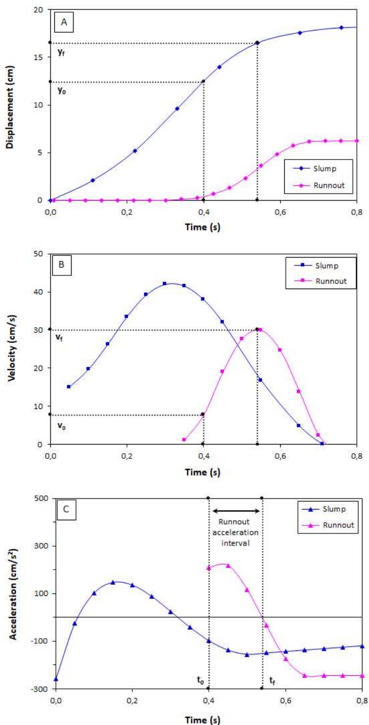
Figure 4. Typical kinematical curves, for both runout and slump movements, obtained in the slump test. (A) Displacement-time curves. (B) Velocity-time curves. (C) Acceleration-time curves.
