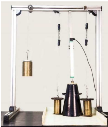
Figure 3. Modified slump test set-up.
