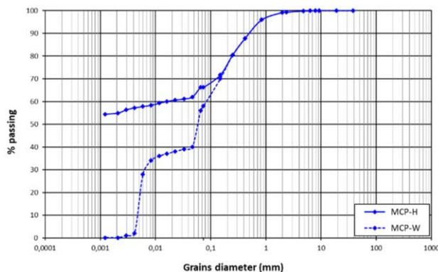
Figure 2. Grain size distribution of the MCP soil. Sedimentation tests performed with both sodium hexametaphosphate (H) and water (W) as deflocculant.
