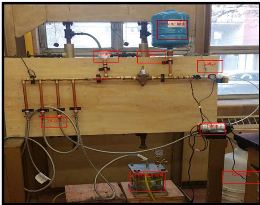
Figure 1. Developed apparatus for leaching samples under constant head conditions.
