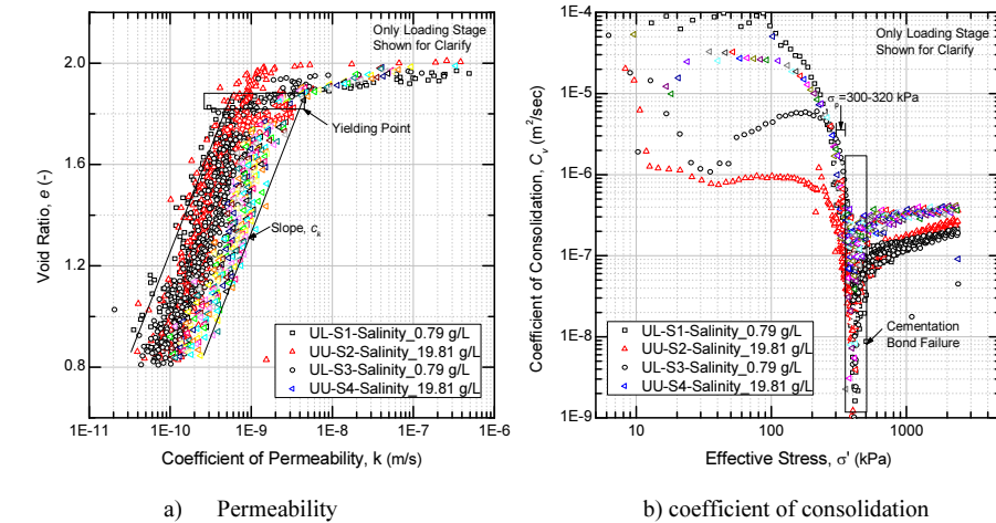
Figure 3. Influence of leaching on the permeability and consolidation coefficient of Champlain Sea clay.
