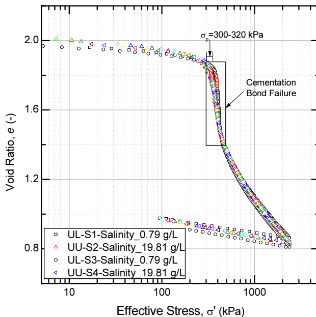
Figure 2. Influence of leaching on e-log p curve of undisturbed Sample.
