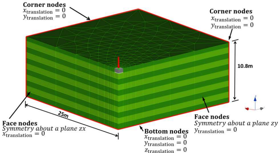
Figure 4. Model of finite elements.
