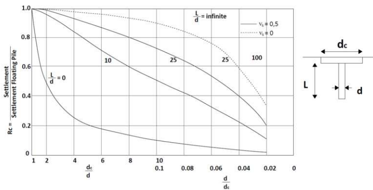
Figure 2. Contact effect of isolate pile [4].
