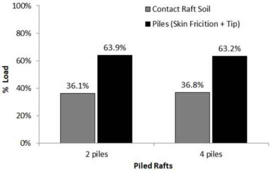
Figure 7. Raft / soil contact distribution.
