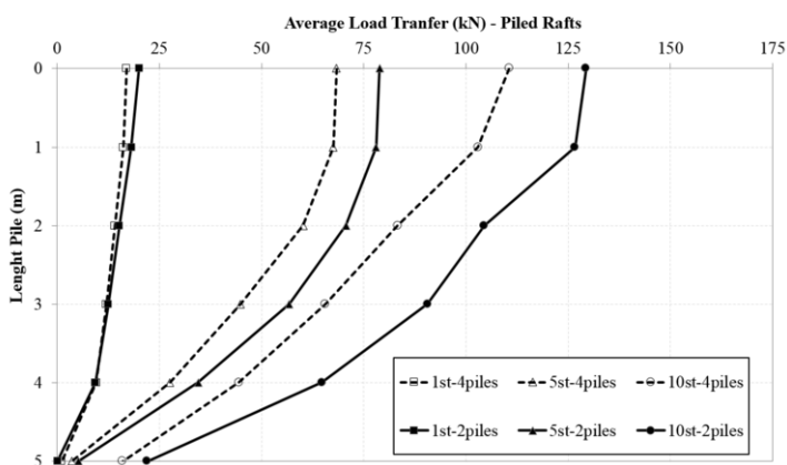
Figure 6. Load transfer curves for piles.
