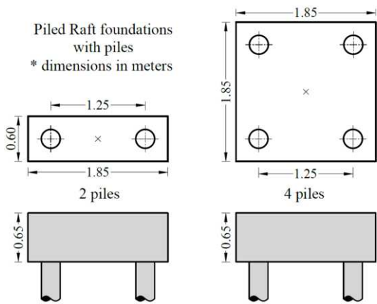
Figure 3. Plan view and elevation details of piled rafts foundations.
