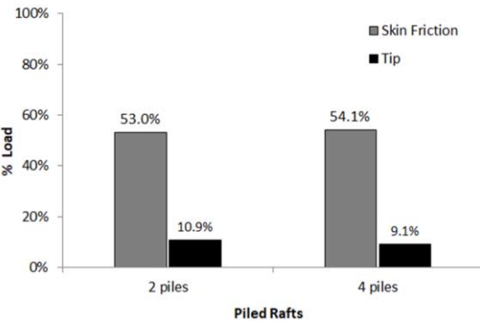
Figure 8. Pile load distribution.
