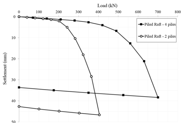
Figure 5. Load vs settlement curve for piled rafts.
