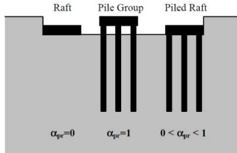
Figure 1. Foundation system [3].
