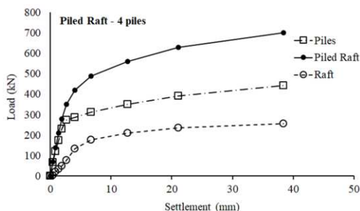
Figure 10. Load vs settlement curves - four piles.
