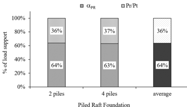
Figure 11. Contribution of the group of piles ( \alpha_{PR} ) and raft / soil contact.
