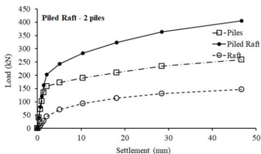
Figure 9. Load vs settlement curves - two piles.
