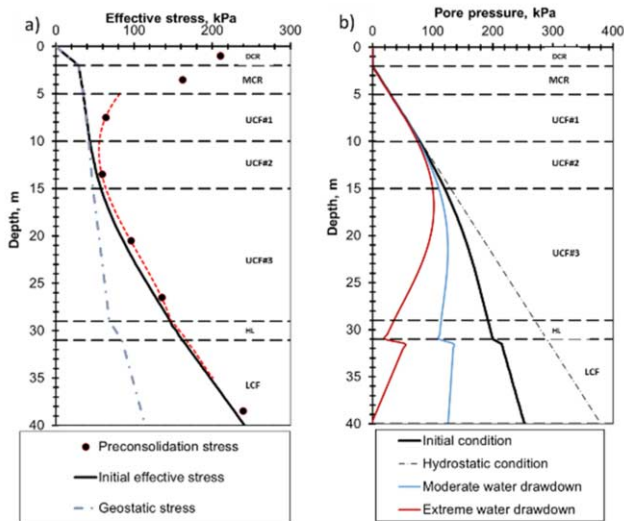
Figure 1. Initial stress state and piezometric conditions.
