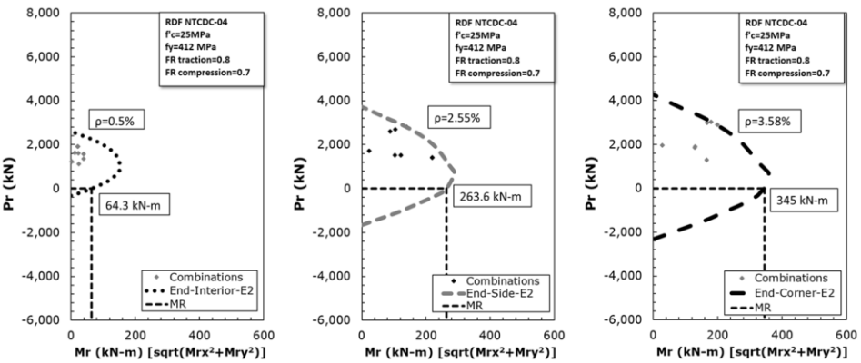
Figure 6. Interaction diagrams for Stage 2 on end-bearing piles.
