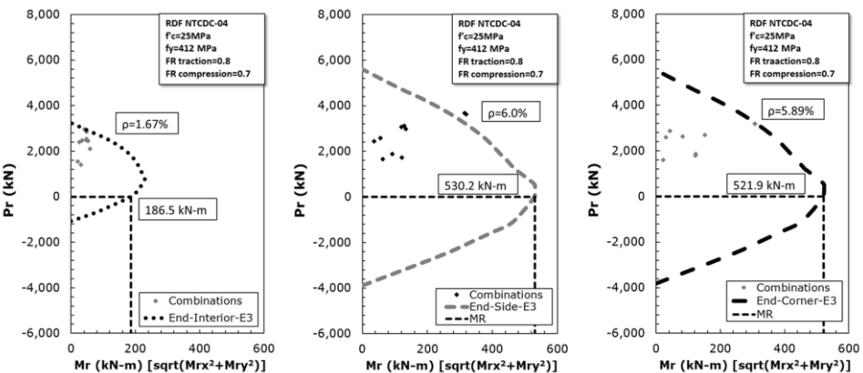
Figure 7. Interaction diagrams for Stage 3 on end-bearing piles.
