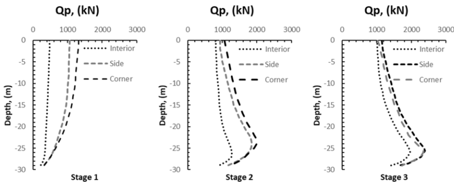
Figure 4. Axial load (Qp) for the different stages in end-bearing piles.
