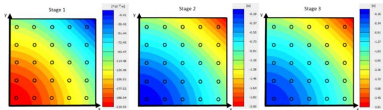
Figure 3. Contour of verticals displacements on the foundation slab for the different stages.
