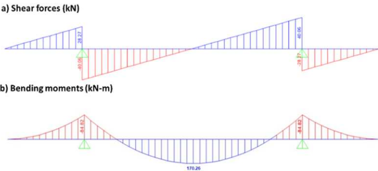
Figure 8. Shear (a) and bending moments (b) diagrams for a configuration of 2 lifting points.
