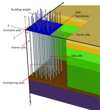
Figure 2. Foundation slab model with end-bearing piles in a FEM 3D program.
