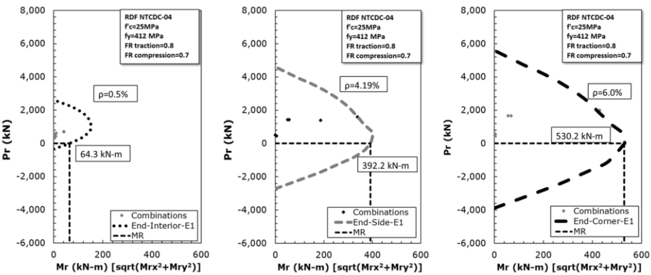
Figure 5. Interaction diagrams for Stage 1 on end-bearing piles.
