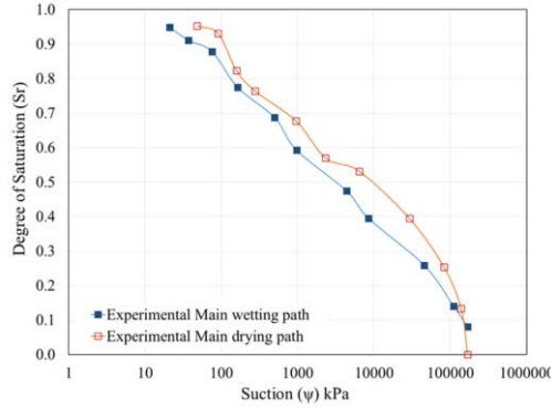
Figure 1. Soil-Water Retention Curve of Jurica's expansive soil.
